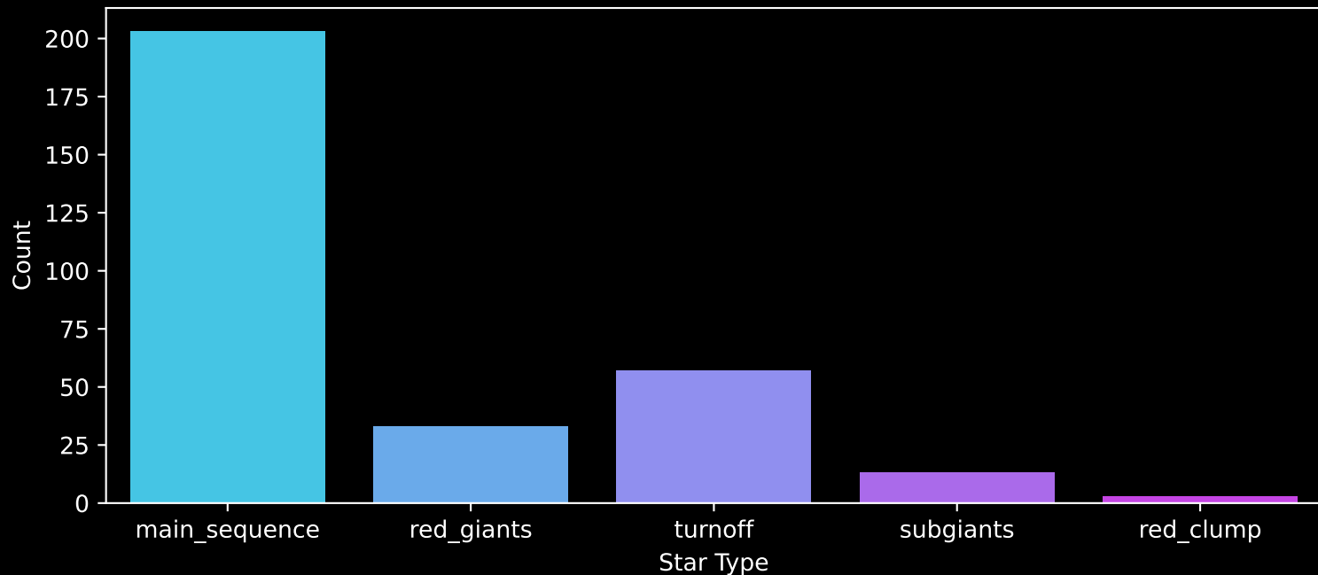
GALAH DR4 Field: [6959] Count plot of Star Type
