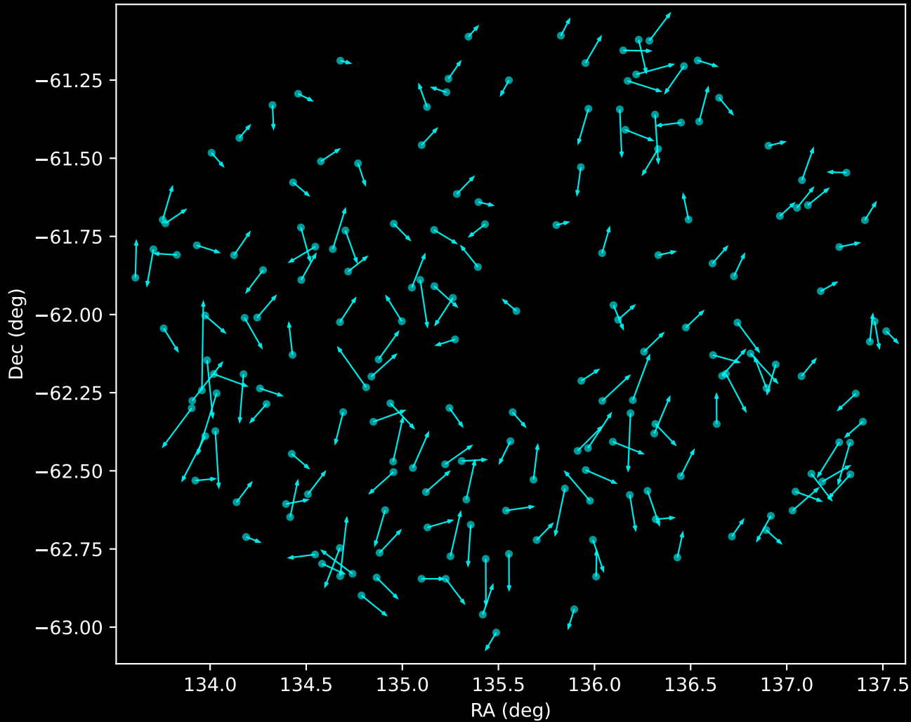
GALAH DR4 Noise Stream Proper Motion Vectors (n=183)
