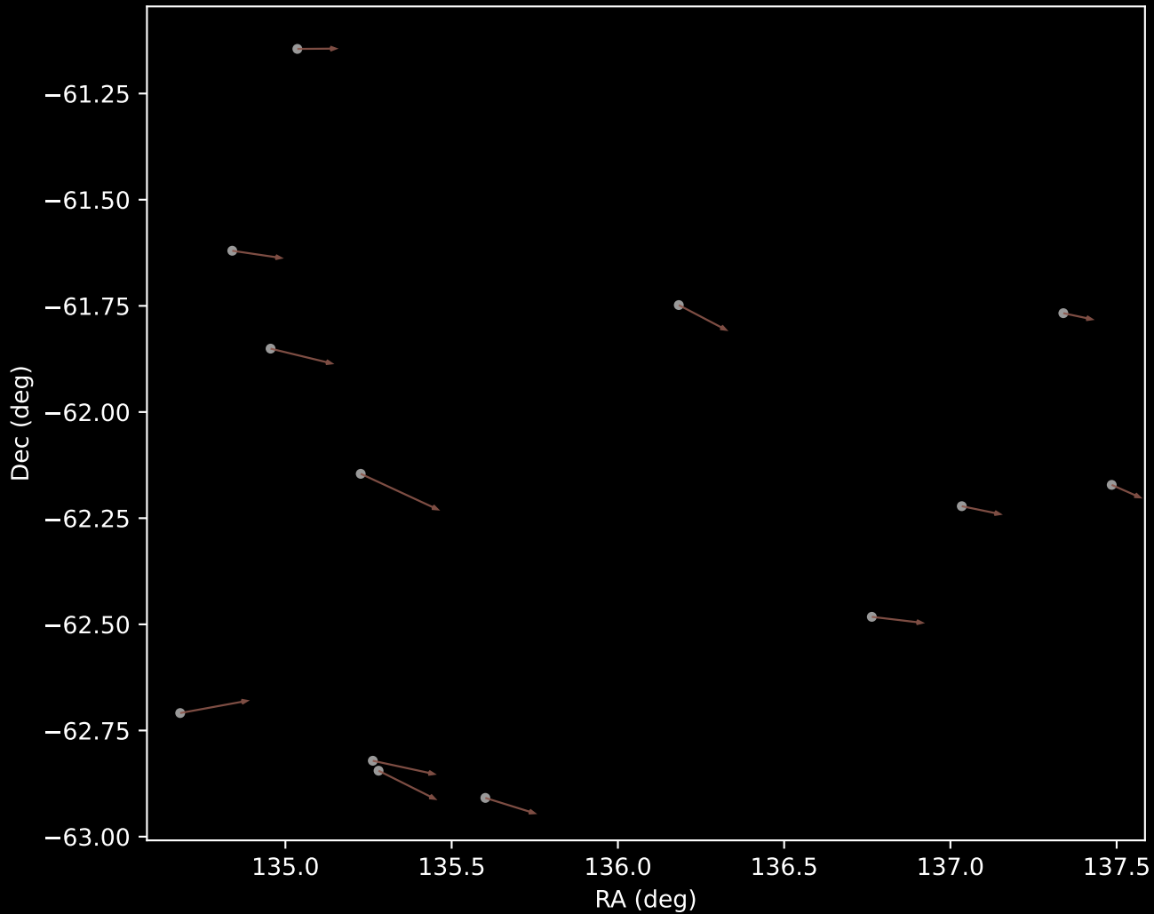
GALAH DR4 Cluster 10 Proper Motion Vectors (n=13)
