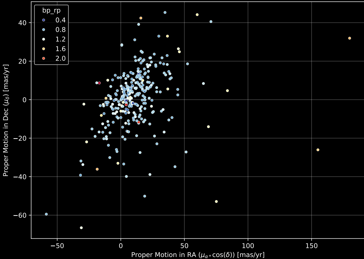
GALAH DR4 Field: [6959] Proper Motion Diagram (n= 309)
