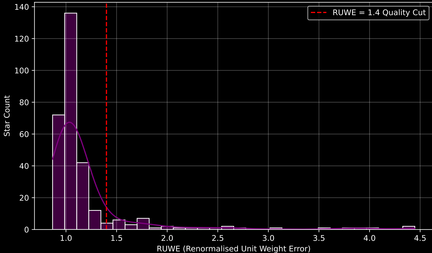
GALAH DR4 Field [6959] RUWE Distribution (n= 299)
